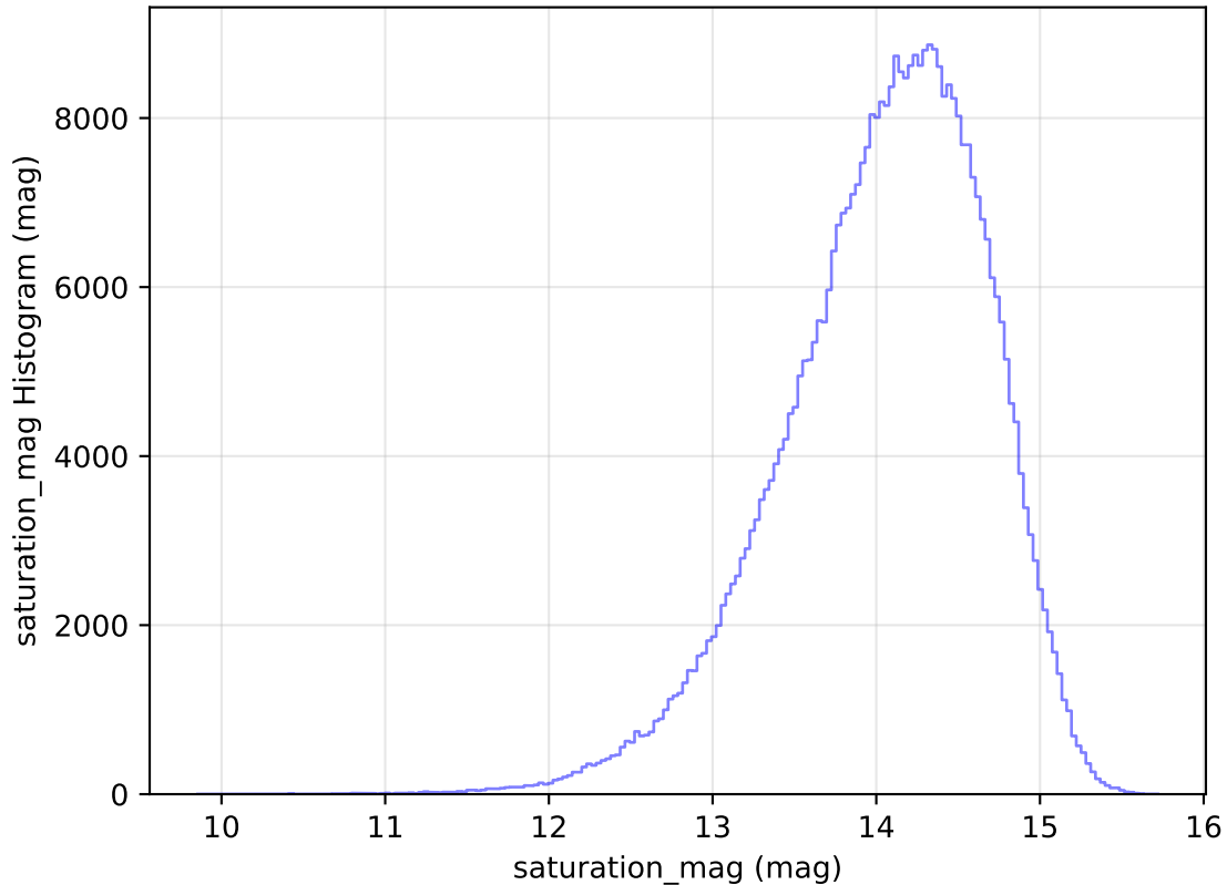
internal_u_expt30_nscale1.0v3.4_10yrs WFD z band: saturation_mag Histogram
