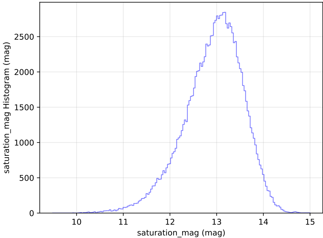
internal_u_expt30_nscale1.0v3.4_10yrs WFD u band: saturation_mag Histogram
