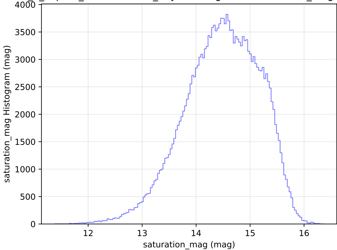
internal_u_expt30_nscale1.0v3.4_10yrs WFD g band: saturation_mag Histogram
