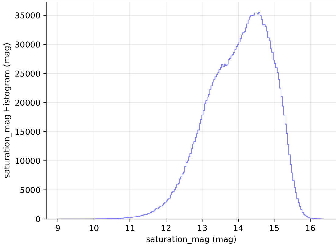
internal_u_expt30_nscale1.0v3.4_10yrs WFD all bands: saturation_mag Histogram
