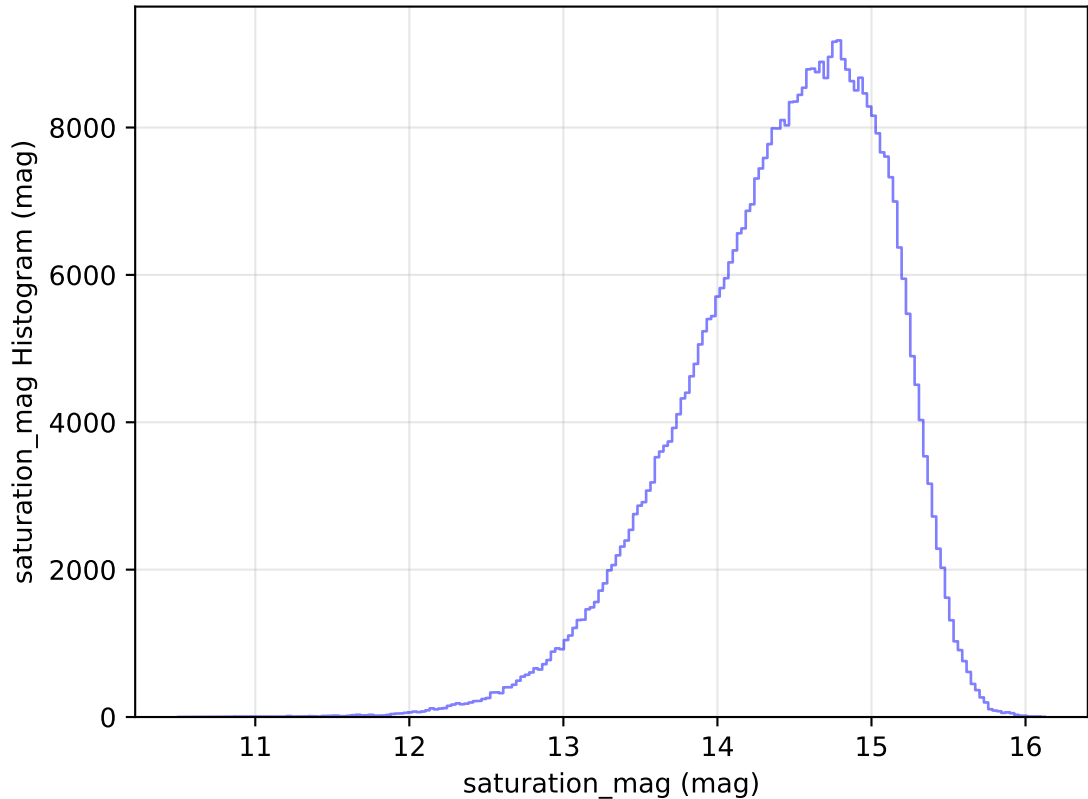
internal_u_expt30_nscale1.0v3.4_10yrs All sky i band: saturation_mag Histogram
