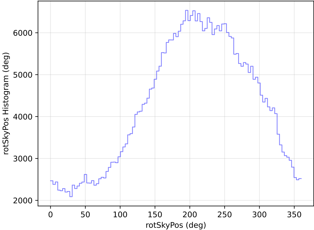
internal_u_expt30_nscale1.0v3.4_10yrs WFD z band: rotSkyPos Histogram
