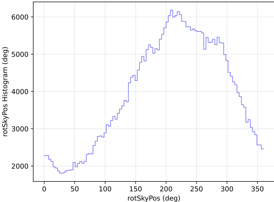
internal_u_expt30_nscale1.0v3.4_10yrs WFD y band: rotSkyPos Histogram
