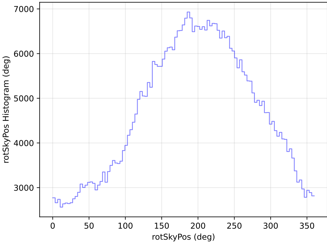
internal_u_expt30_nscale1.0v3.4_10yrs WFD r band: rotSkyPos Histogram
