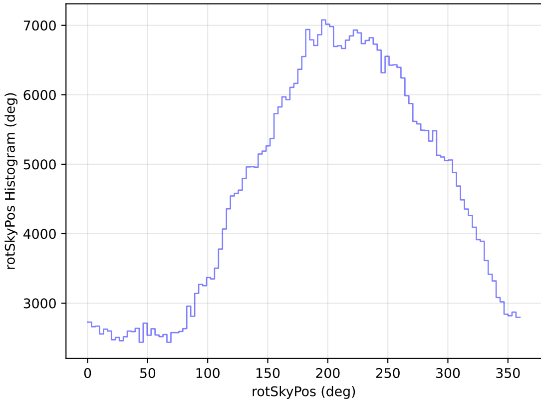
internal_u_expt30_nscale1.0v3.4_10yrs WFD i band: rotSkyPos Histogram
