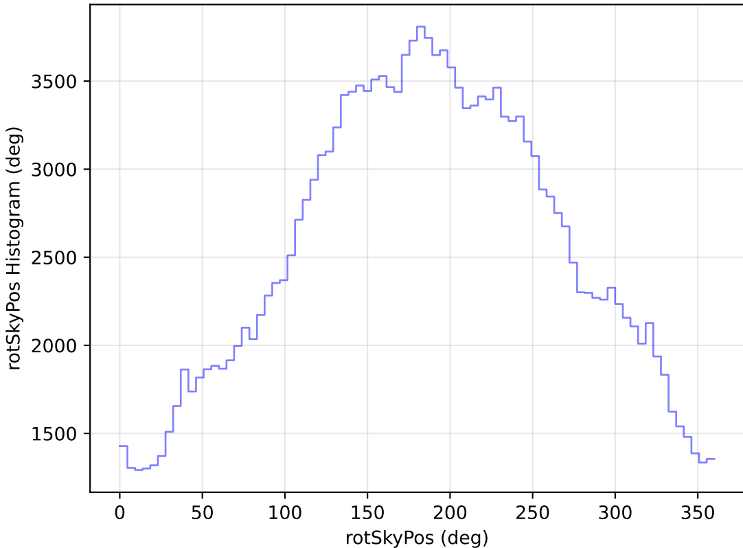
internal_u_expt30_nscale1.0v3.4_10yrs WFD g band: rotSkyPos Histogram
