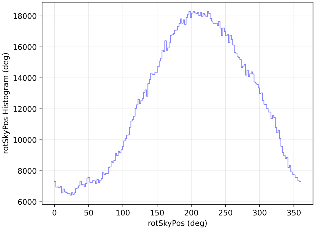
internal_u_expt30_nscale1.0v3.4_10yrs WFD all bands: rotSkyPos Histogram
