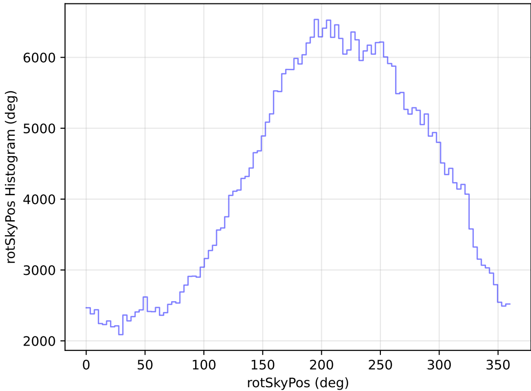
internal_u_expt30_nscale1.0v3.4_10yrs All sky z band: rotSkyPos Histogram
