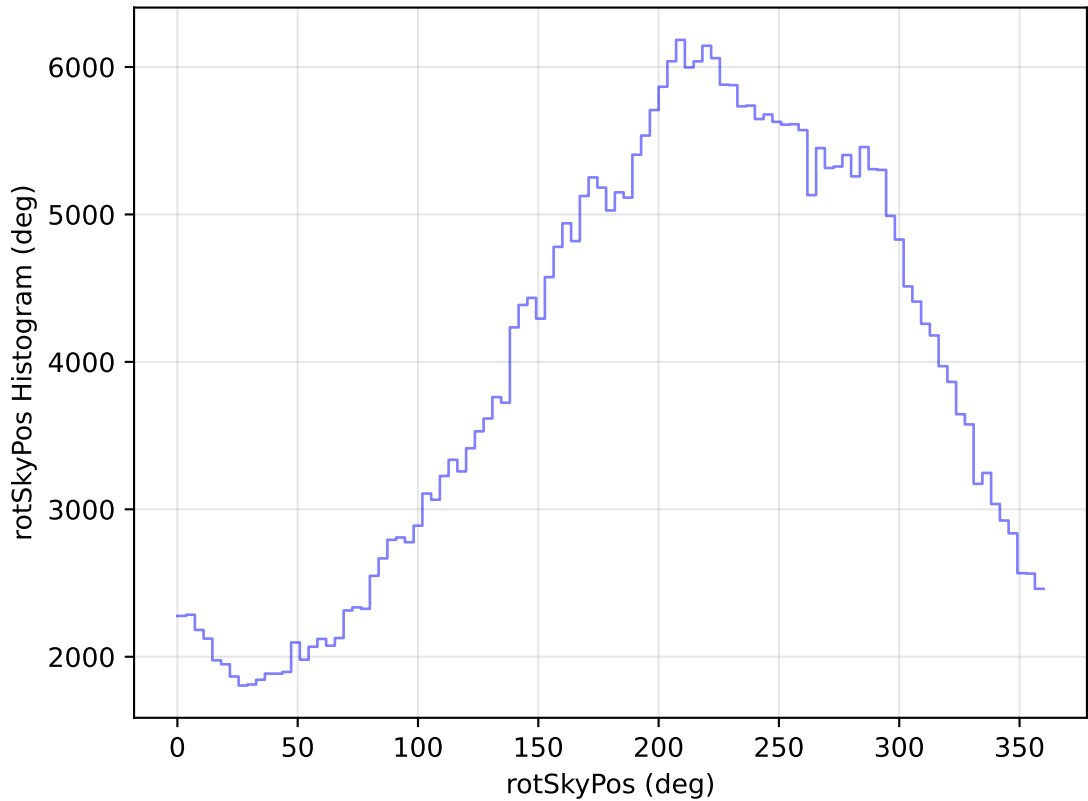
internal_u_expt30_nscale1.0v3.4_10yrs All sky y band: rotSkyPos Histogram
