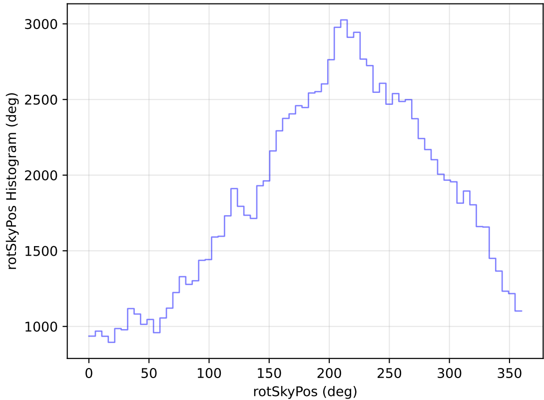
internal_u_expt30_nscale1.0v3.4_10yrs All sky u band: rotSkyPos Histogram
