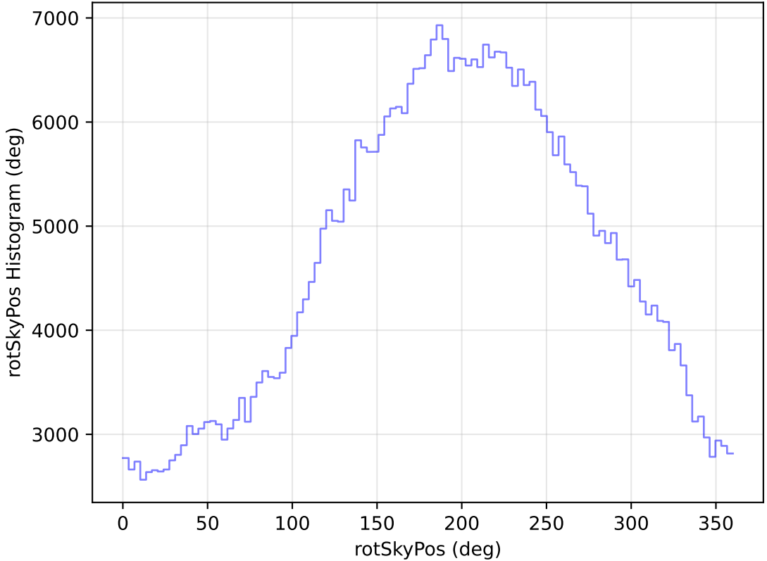
internal_u_expt30_nscale1.0v3.4_10yrs All sky r band: rotSkyPos Histogram
