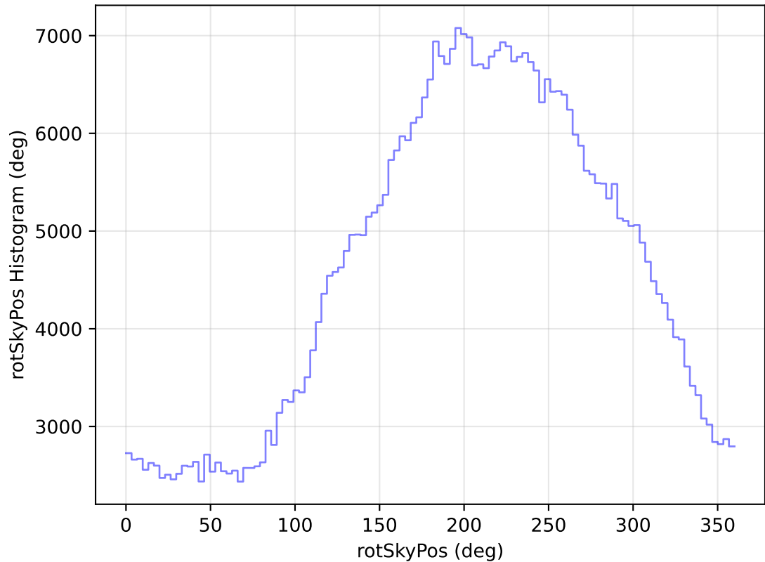
internal_u_expt30_nscale1.0v3.4_10yrs All sky i band: rotSkyPos Histogram
