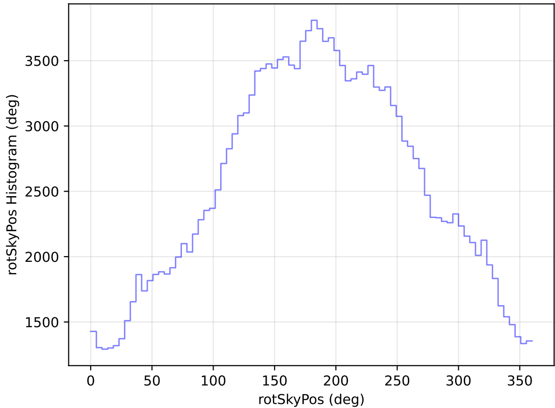
internal_u_expt30_nscale1.0v3.4_10yrs All sky g band: rotSkyPos Histogram
