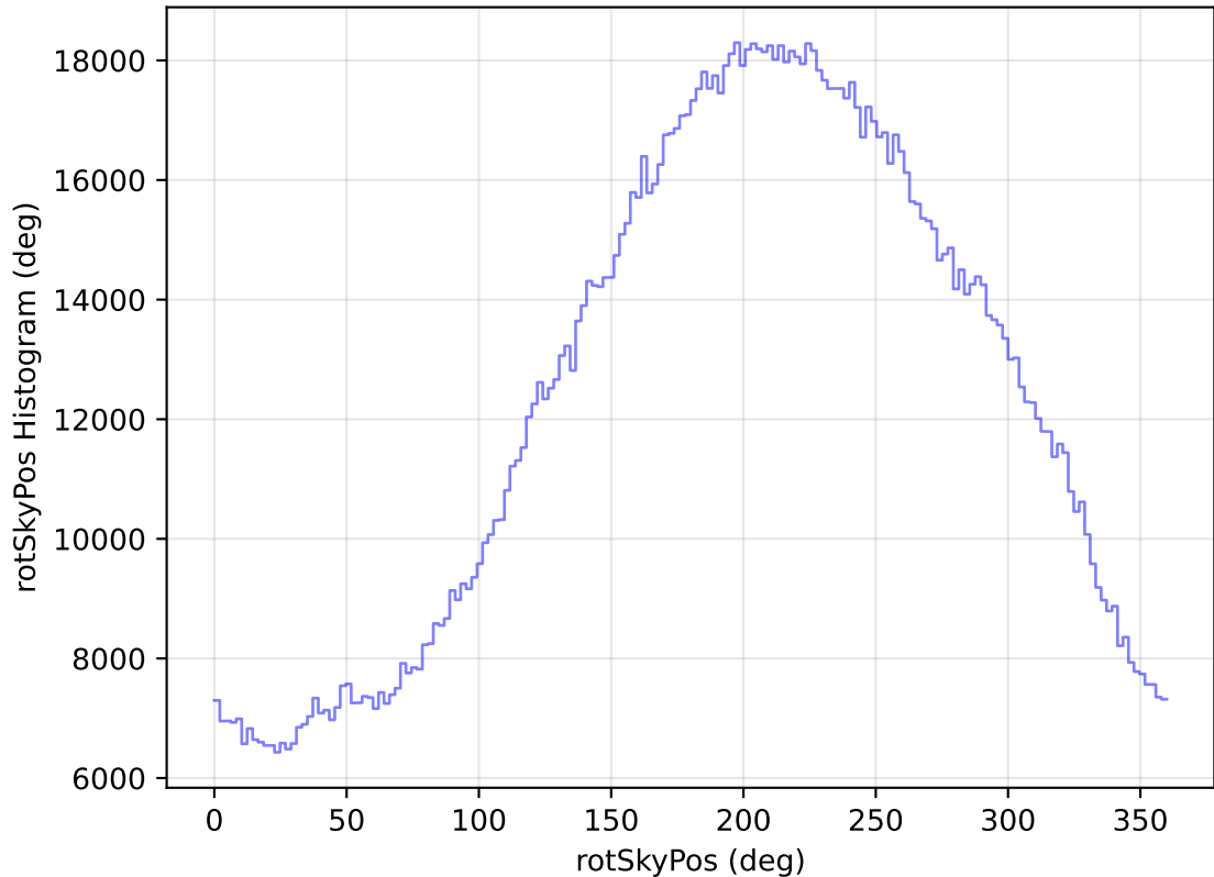
internal_u_expt30_nscale1.0v3.4_10yrs All sky all bands: rotSkyPos Histogram
