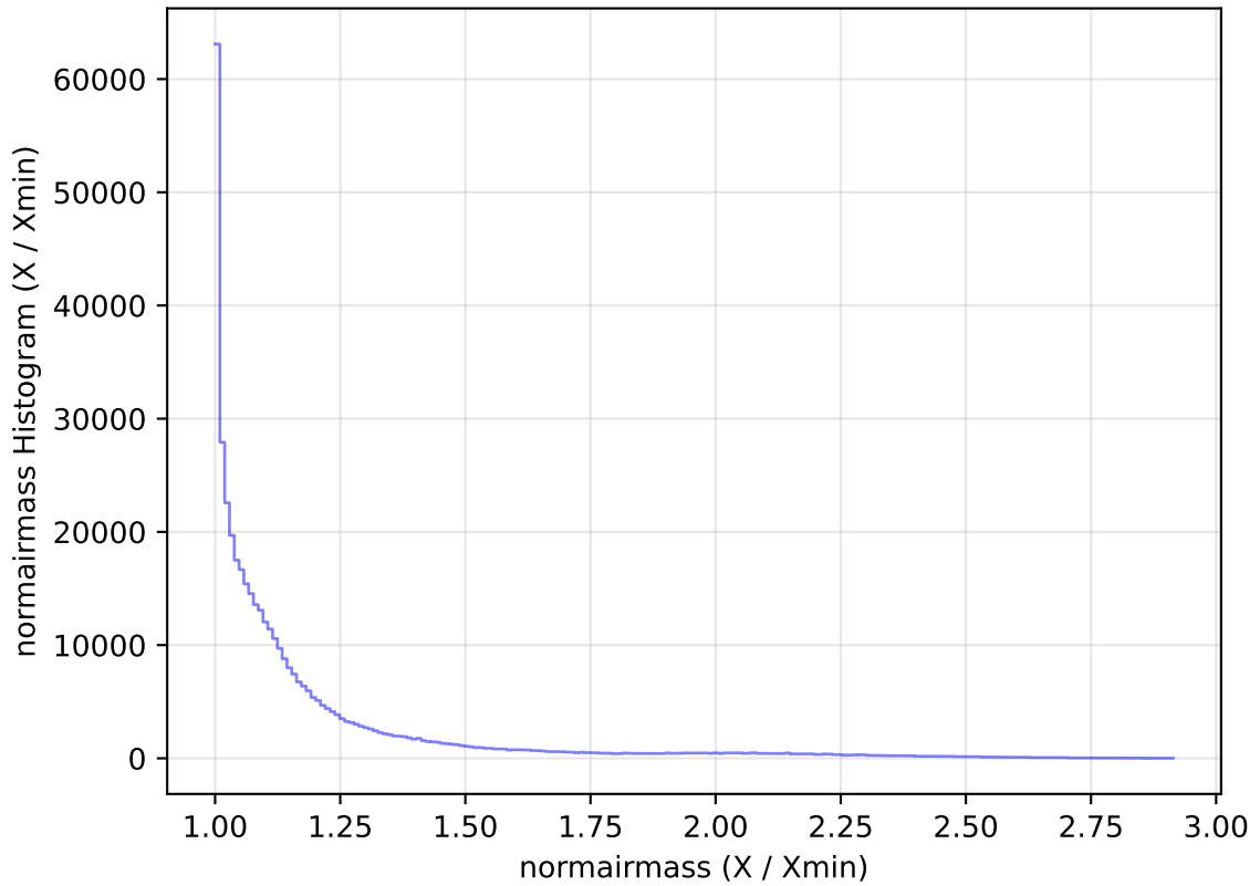
internal_u_expt30_nscale1.0v3.4_10yrs WFD z band: normairmass Histogram
