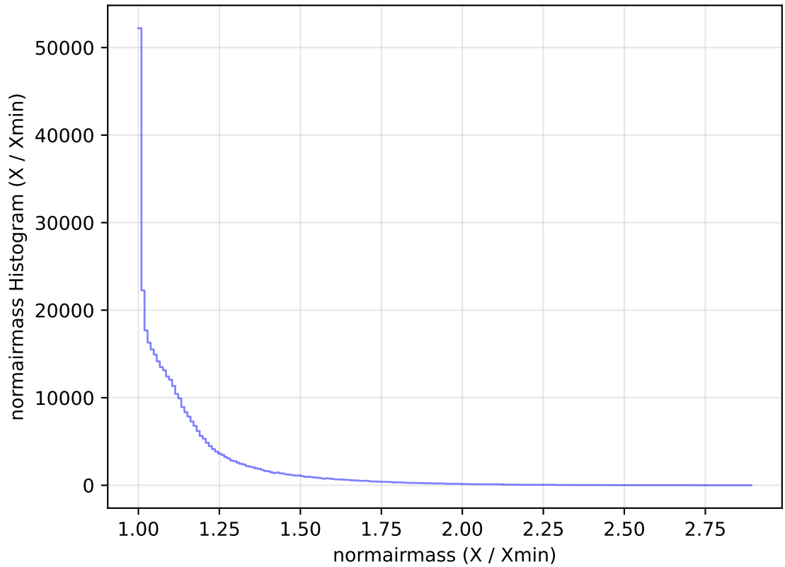
internal_u_expt30_nscale1.0v3.4_10yrs WFD y band: normairmass Histogram
