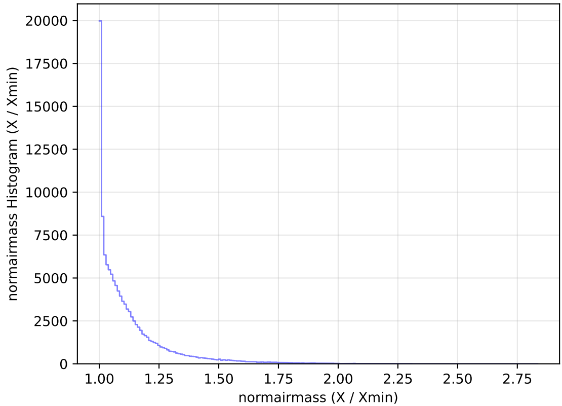
internal_u_expt30_nscale1.0v3.4_10yrs WFD u band: normairmass Histogram
