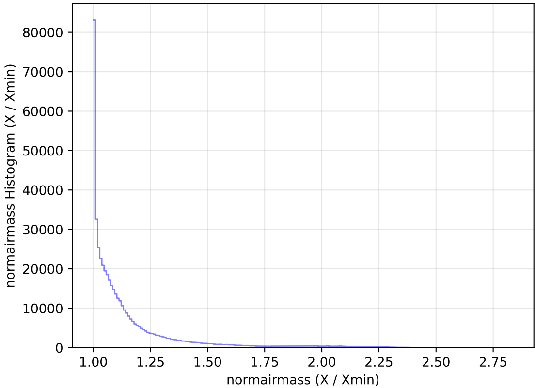
internal_u_expt30_nscale1.0v3.4_10yrs WFD r band: normairmass Histogram
