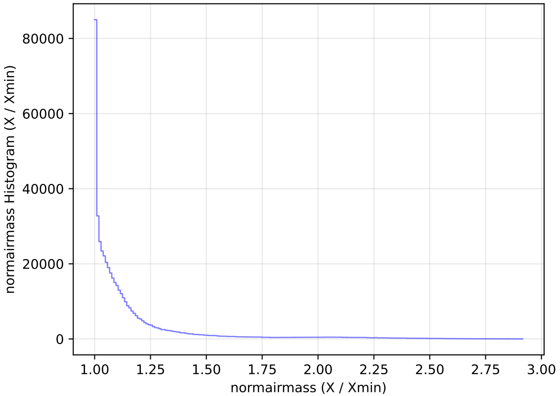
internal_u_expt30_nscale1.0v3.4_10yrs WFD i band: normairmass Histogram
