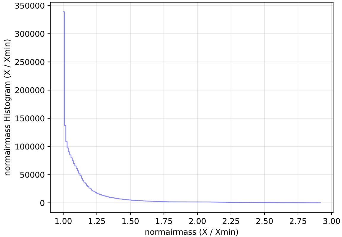
internal_u_expt30_nscale1.0v3.4_10yrs WFD all bands: normairmass Histogram
