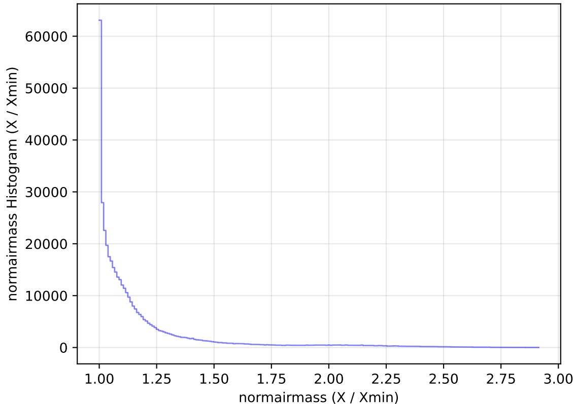
internal_u_expt30_nscale1.0v3.4_10yrs All sky z band: normairmass Histogram
