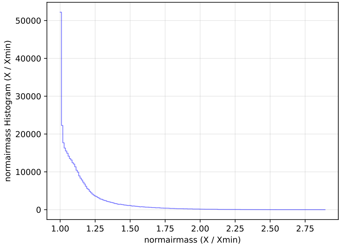
internal_u_expt30_nscale1.0v3.4_10yrs All sky y band: normairmass Histogram
