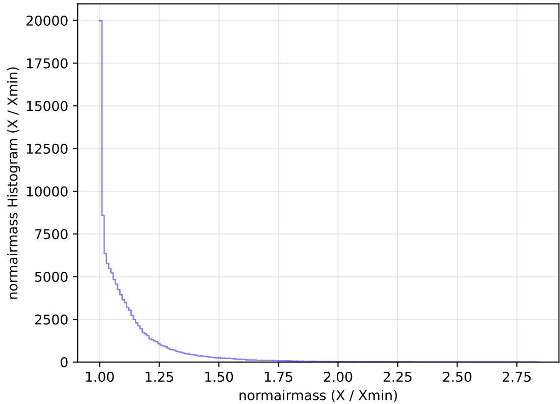
internal_u_expt30_nscale1.0v3.4_10yrs All sky u band: normairmass Histogram
