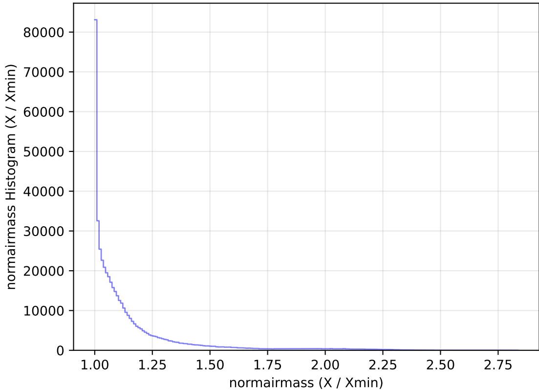
internal_u_expt30_nscale1.0v3.4_10yrs All sky r band: normairmass Histogram
