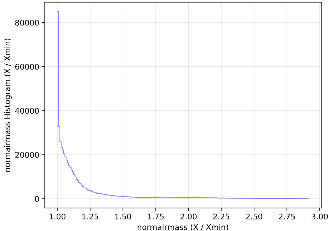
internal_u_expt30_nscale1.0v3.4_10yrs All sky i band: normairmass Histogram
