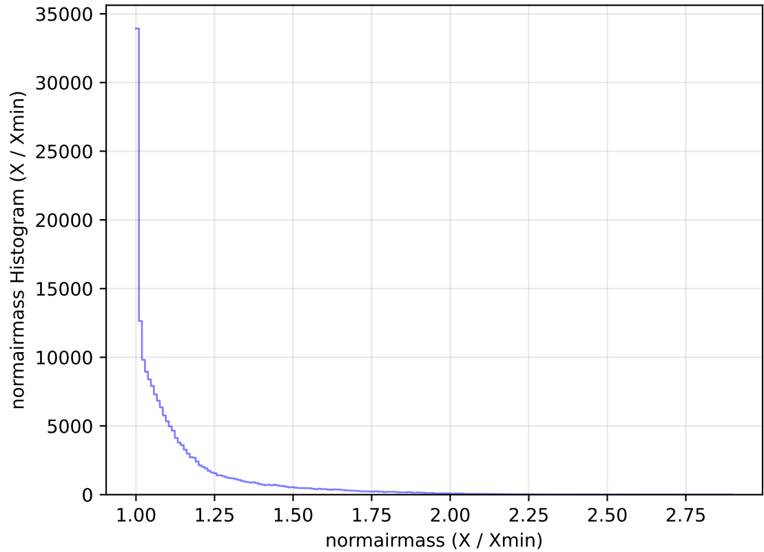
internal_u_expt30_nscale1.0v3.4_10yrs All sky g band: normairmass Histogram
