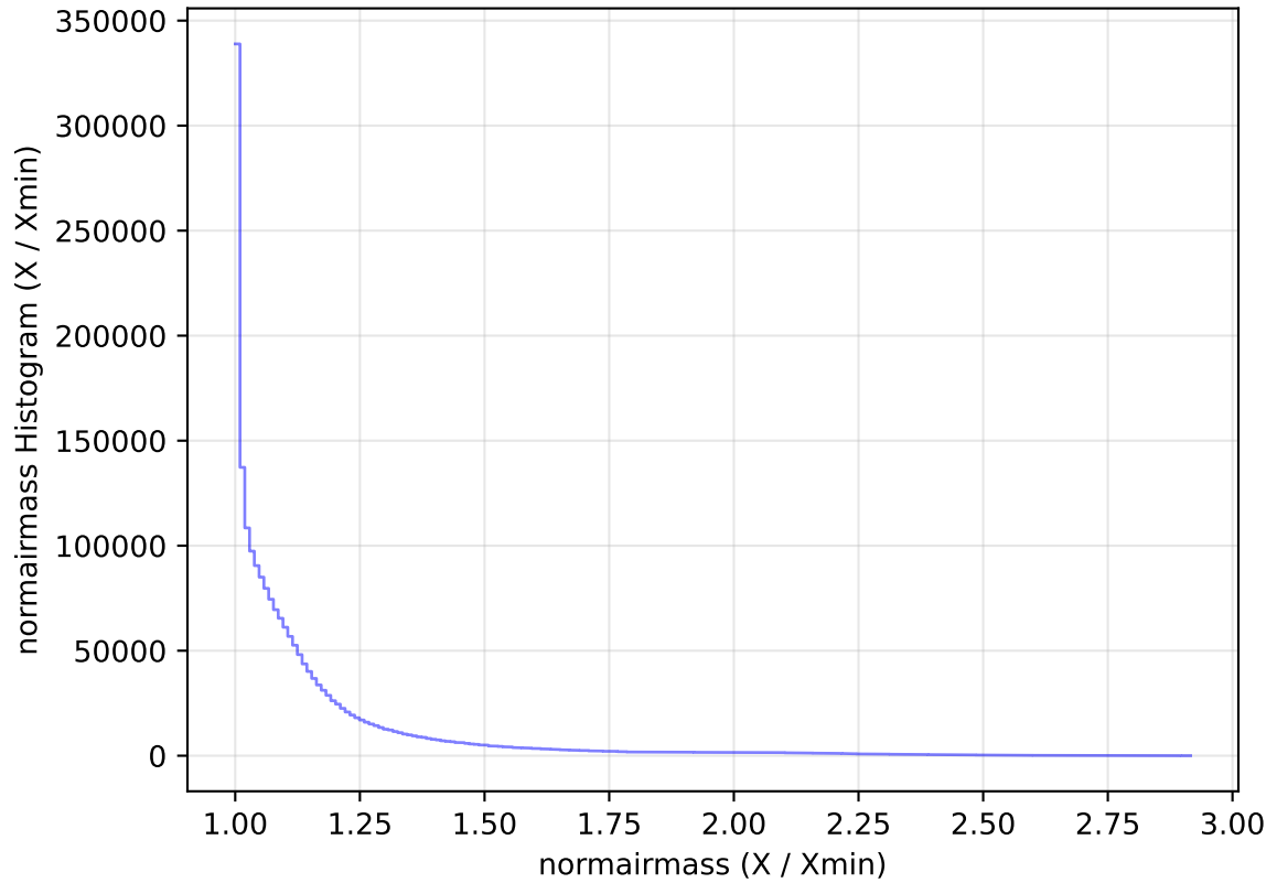
internal_u_expt30_nscale1.0v3.4_10yrs All sky all bands: normairmass Histogram
