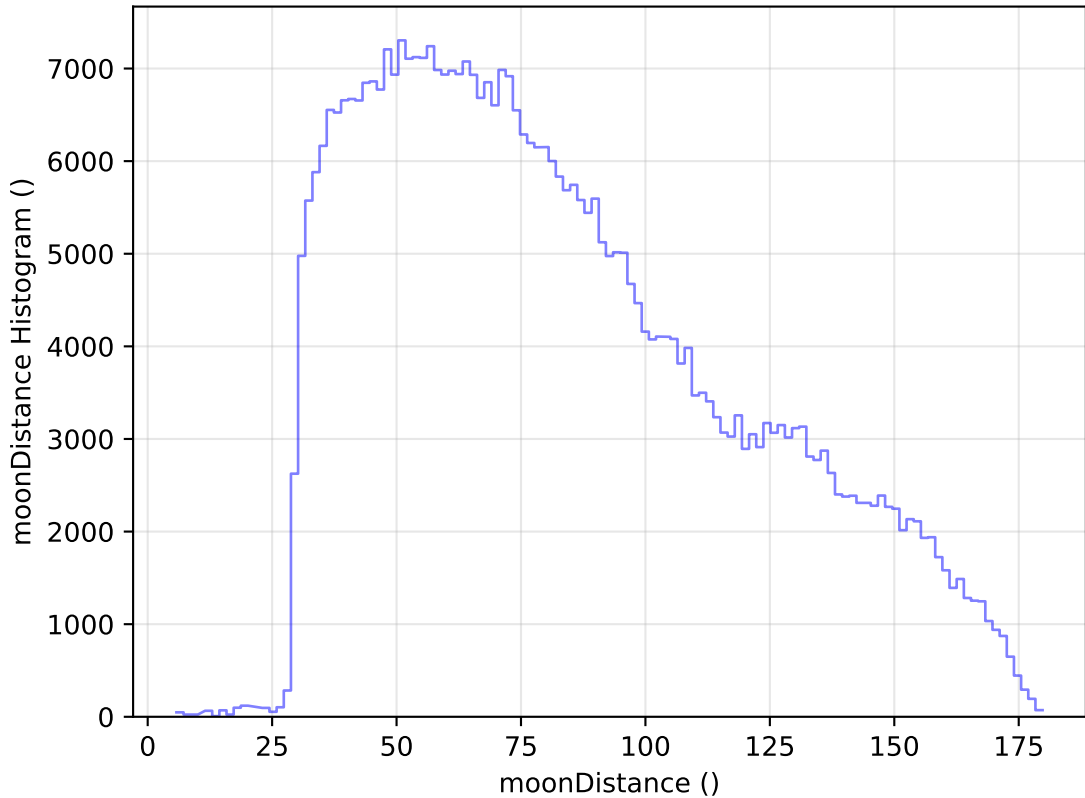
internal_u_expt30_nscale1.0v3.4_10yrs WFD z band: moonDistance Histogram
