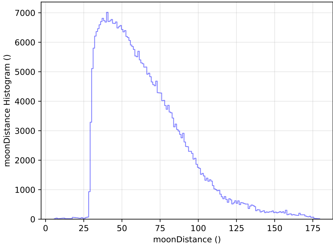
internal_u_expt30_nscale1.0v3.4_10yrs WFD y band: moonDistance Histogram
