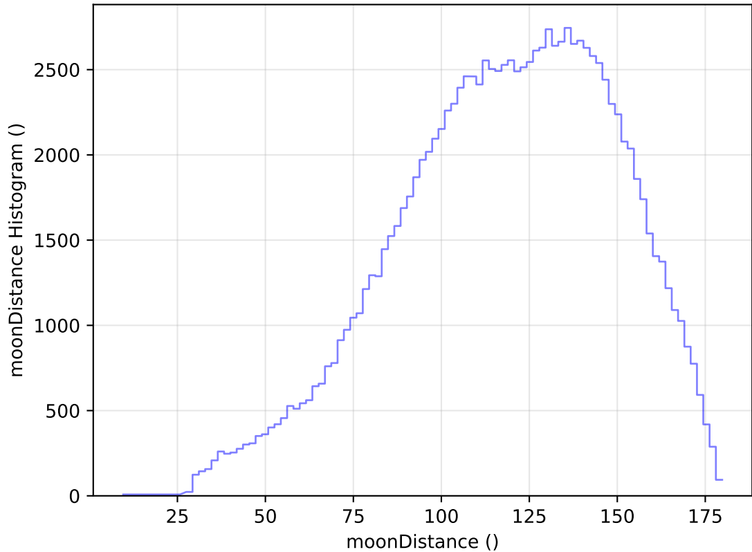
internal_u_expt30_nscale1.0v3.4_10yrs WFD u band: moonDistance Histogram
