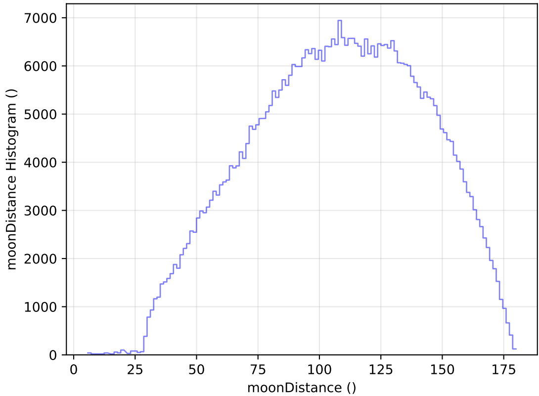
internal_u_expt30_nscale1.0v3.4_10yrs WFD r band: moonDistance Histogram
