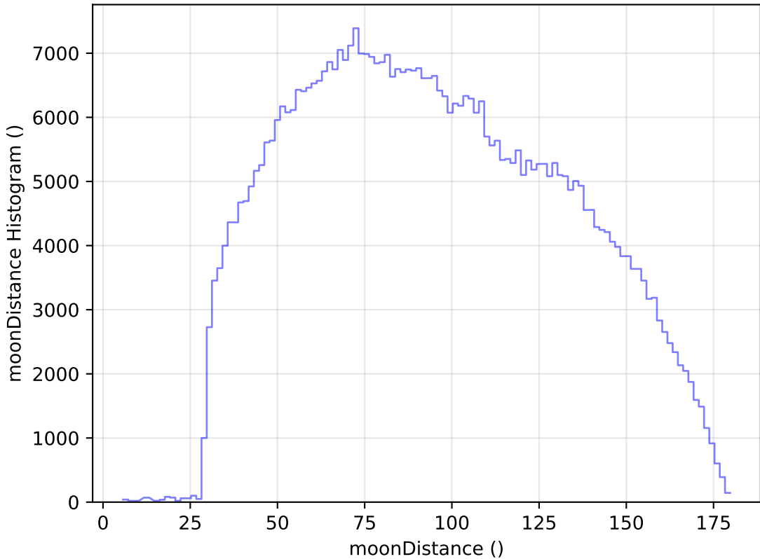
internal_u_expt30_nscale1.0v3.4_10yrs WFD i band: moonDistance Histogram
