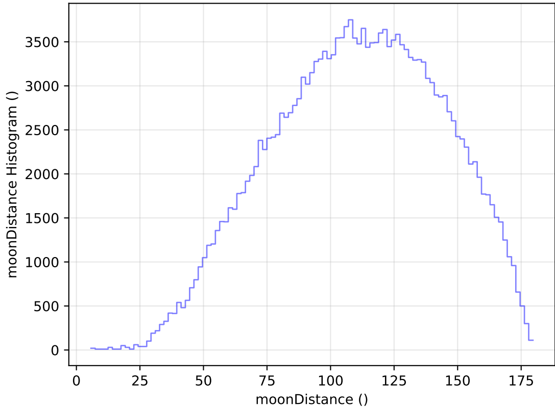
internal_u_expt30_nscale1.0v3.4_10yrs WFD g band: moonDistance Histogram
