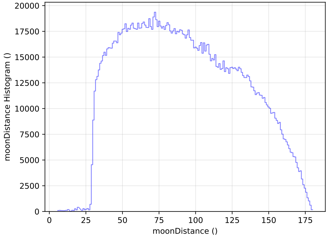
internal_u_expt30_nscale1.0v3.4_10yrs WFD all bands: moonDistance Histogram
