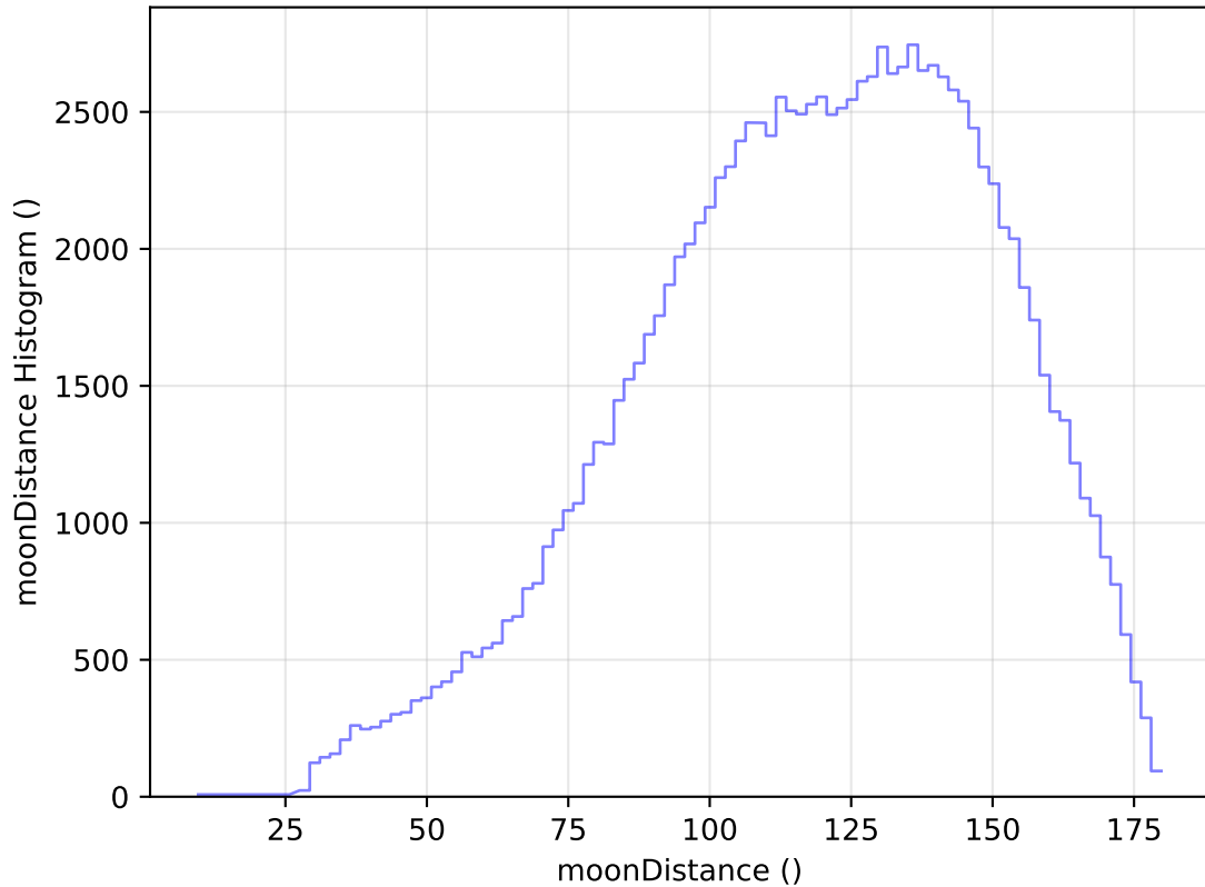
internal_u_expt30_nscale1.0v3.4_10yrs All sky u band: moonDistance Histogram
