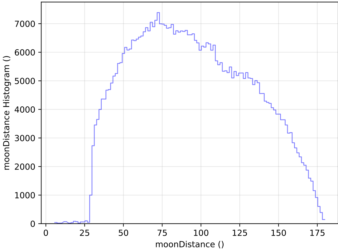
internal_u_expt30_nscale1.0v3.4_10yrs All sky i band: moonDistance Histogram
