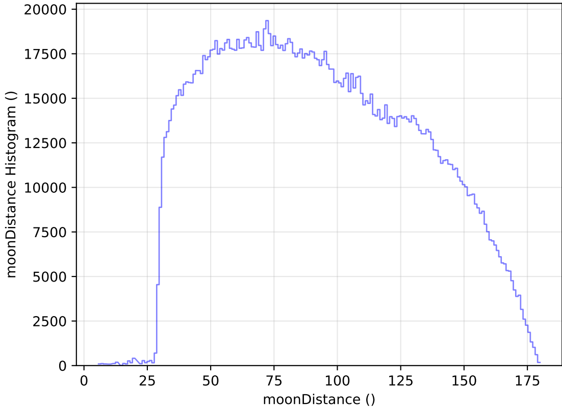
internal_u_expt30_nscale1.0v3.4_10yrs All sky all bands: moonDistance Histogram
