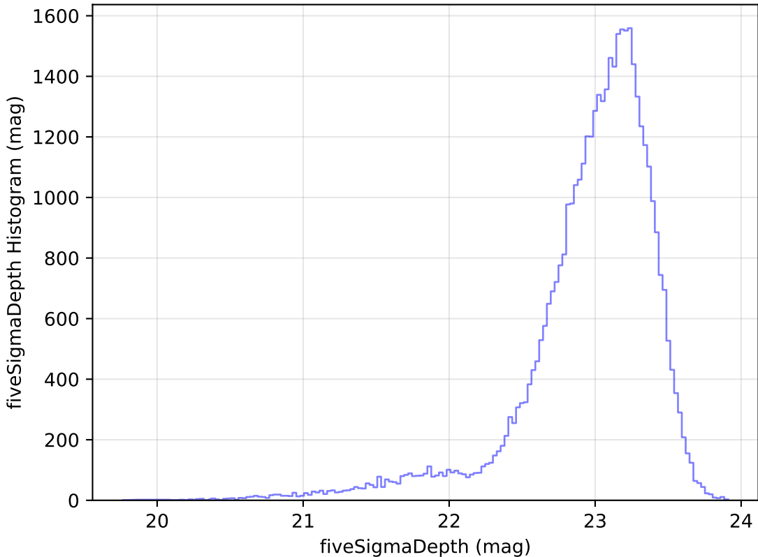
internal_u_expt30_nscale1.0v3.4_10yrs Yr 1 z band: fiveSigmaDepth Histogram
