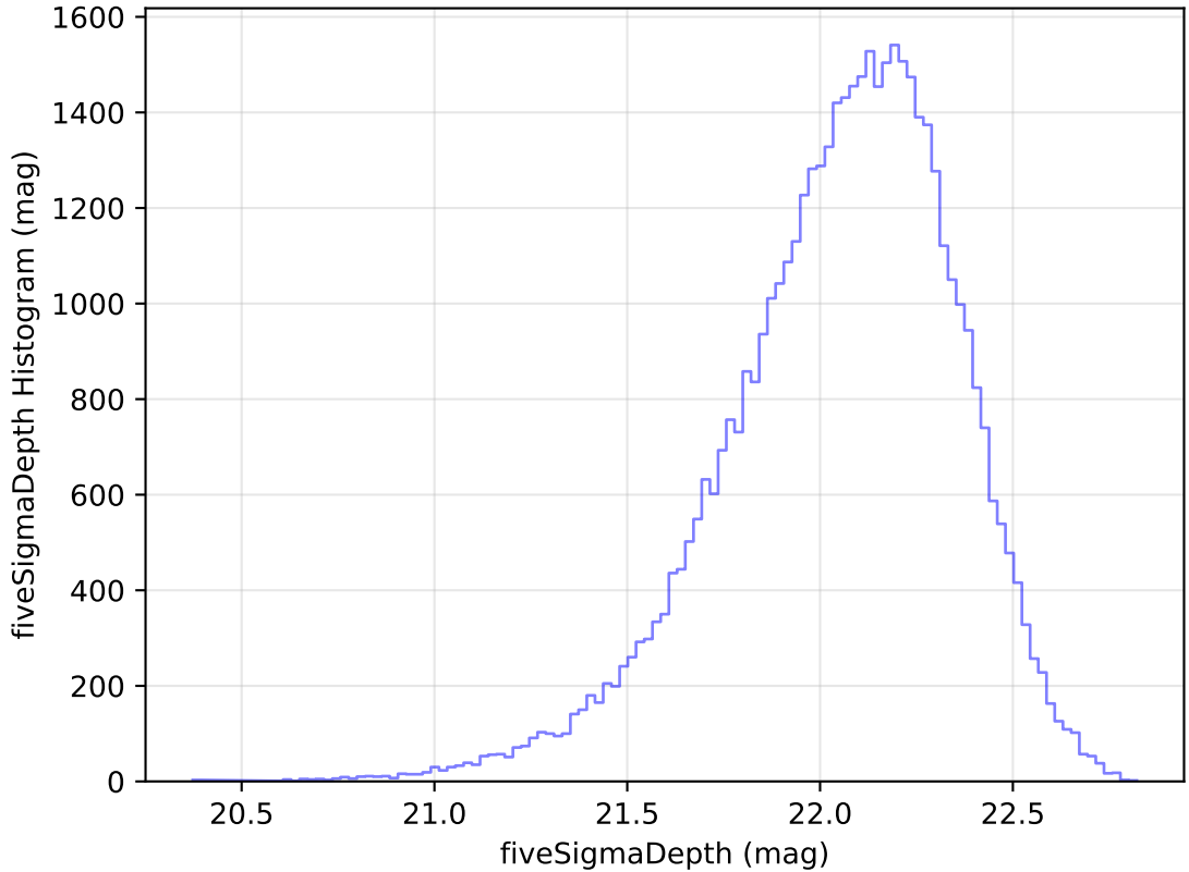
internal_u_expt30_nscale1.0v3.4_10yrs Yr 1 y band: fiveSigmaDepth Histogram
