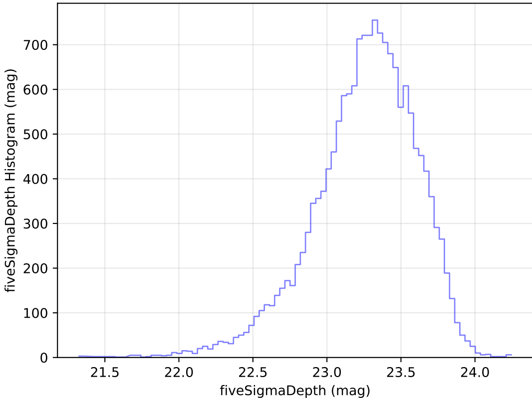
internal_u_expt30_nscale1.0v3.4_10yrs Yr 1 u band: fiveSigmaDepth Histogram
