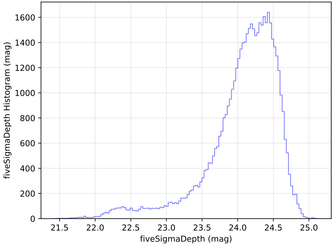
internal_u_expt30_nscale1.0v3.4_10yrs Yr 1 r band: fiveSigmaDepth Histogram
