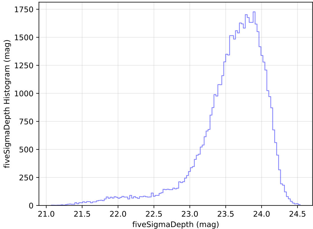
internal_u_expt30_nscale1.0v3.4_10yrs Yr 1 i band: fiveSigmaDepth Histogram
