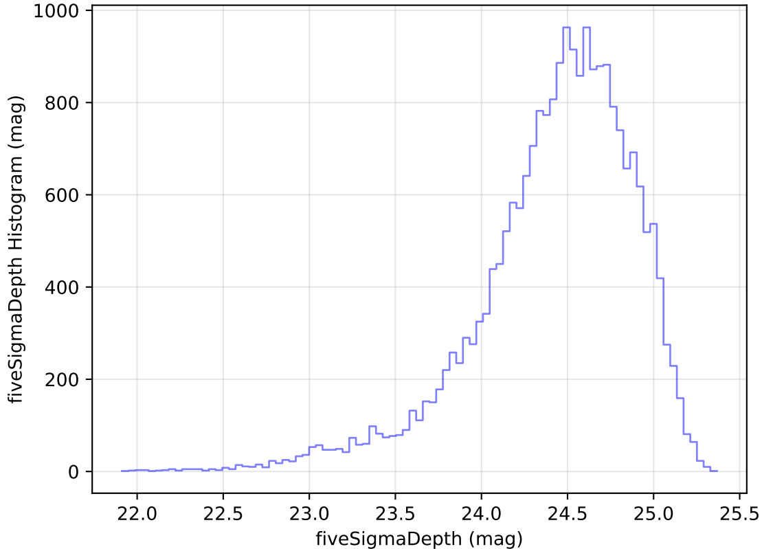
internal_u_expt30_nscale1.0v3.4_10yrs Yr 1 g band: fiveSigmaDepth Histogram
