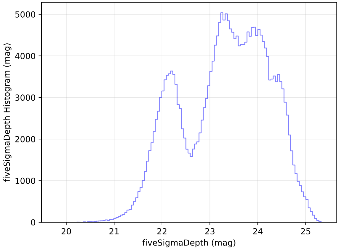
internal_u_expt30_nscale1.0v3.4_10yrs Yr 1 all bands: fiveSigmaDepth Histogram
