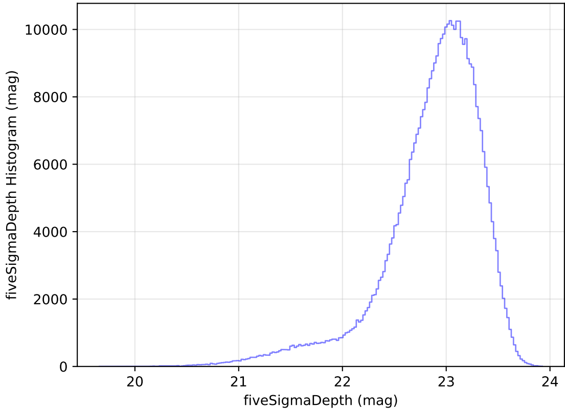
internal_u_expt30_nscale1.0v3.4_10yrs WFD z band: fiveSigmaDepth Histogram
