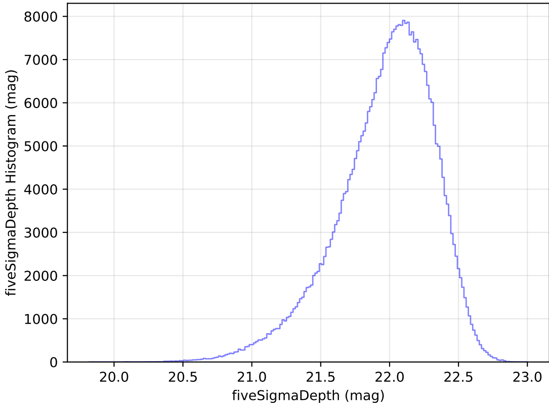
internal_u_expt30_nscale1.0v3.4_10yrs WFD y band: fiveSigmaDepth Histogram
